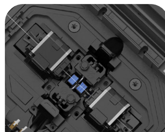
Bare Fiber
