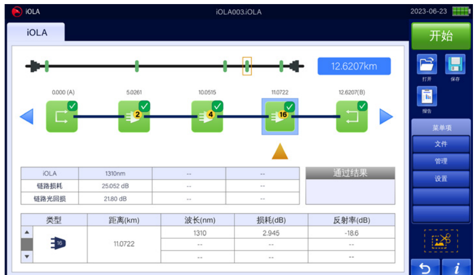
Measuring total 1:128 splitter
