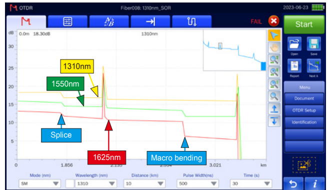
A trace with a macro bend
